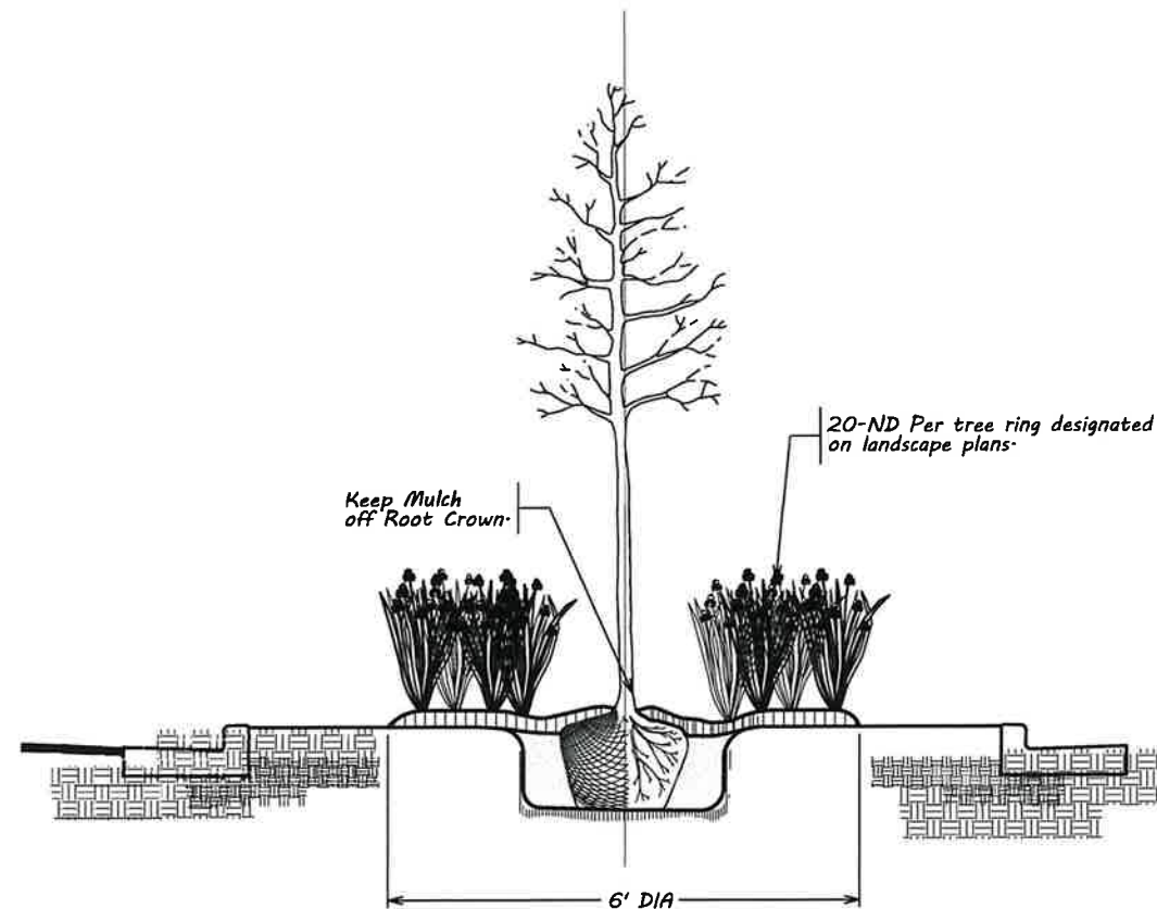
Tree Ring Sectional (TYPICAL) No Scale
