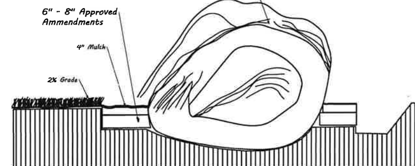
Typical Section @ Boulder Placement No Scale
